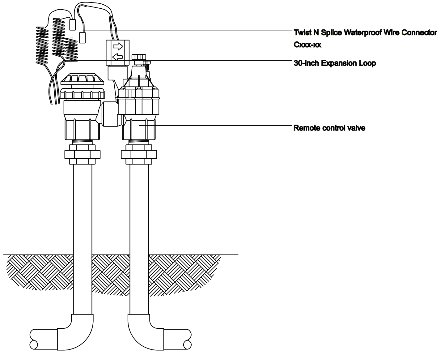
Antisiphon Valve Assembly
